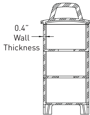
Cross-Section of Enclosure
