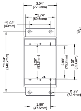
Single-Gang Front View
