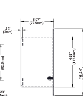
Single-Gang Side View
