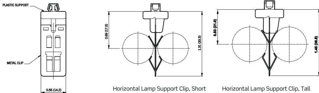
Horizontal Lamp Support Clips 23452-MTS, 234452-MTL
