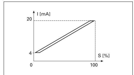
Figure 1. Analog Output
