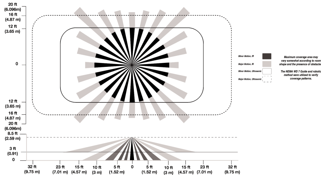
OAC-DT-2000-R Coverage Diagram
